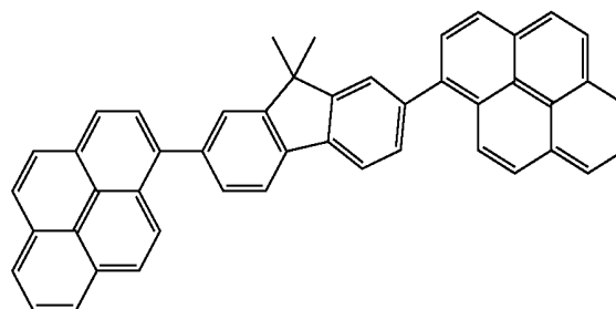
Compound 9
