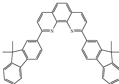
Compound 5
