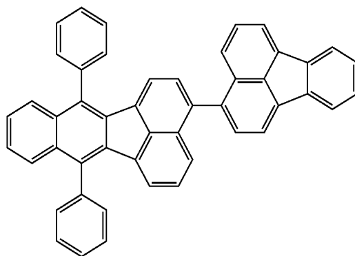
Compound 3
