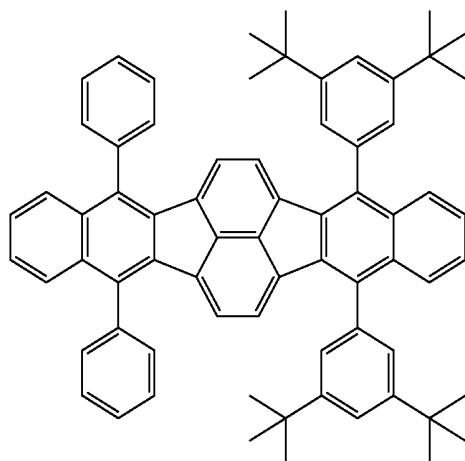
Compound 10
