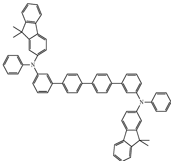
Compound 1
