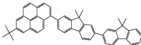
Compound 3
